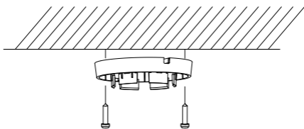
Figure 2-3 Install the Mounting Base to Wooden Ceiling
