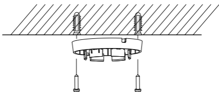
Figure 2-4 Install the Mounting Base to Cement Ceiling
