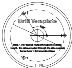
Figure 2-2 Drill Template
