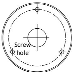
Figure 2-10 Drill Template
