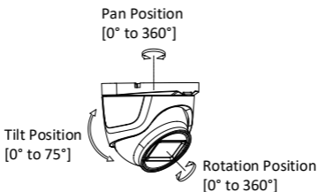
Figure 2-9 3-Axis Adjustment
