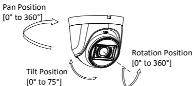
Figure 2-6 3-axis Adjustment
