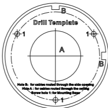
Figure 2-4 Drill Template
