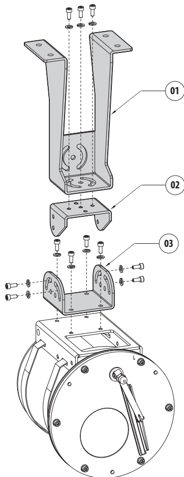
Fig. 10 Ceiling mounting.
