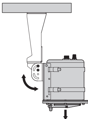
Fig. 16 Example of ceiling installation, vertical rotation, -90°.
