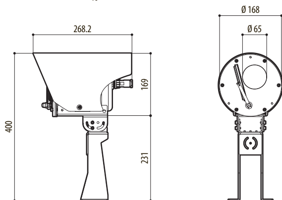
Fig. 46 NVX, parapet mounting.
