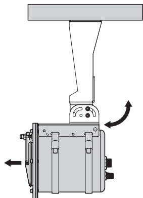
Fig. 15 Example of ceiling installation, vertical rotation, 0°.
