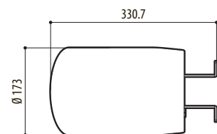
Fig. 45 NVX, wall mounting.
