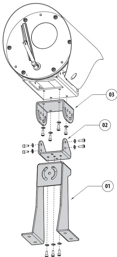
Fig. 9 Parapet mounting.
