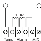
Fully supervised configuration. R1 and R2 to suit the control panel.
