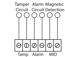
Double pole configuration
