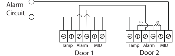
Fully supervised, double door configuration, R1 and R2 to suit control panel
