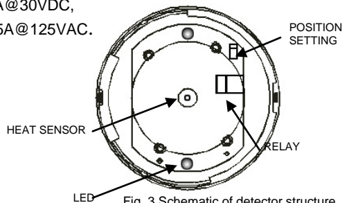
Fig. 3 Schematic of detector structure When front cover is open.
