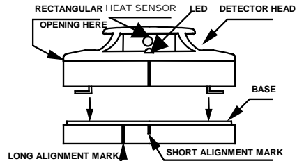
Fig. 2 Mating detector head onto base
