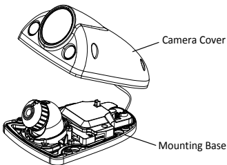
Figure 2-3 Disassemble the Camera
