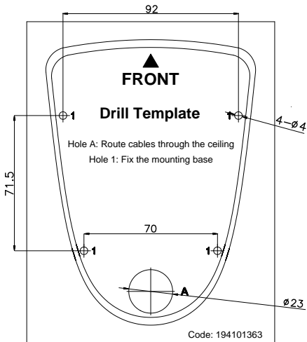
Figure 2-1 Drill Template
