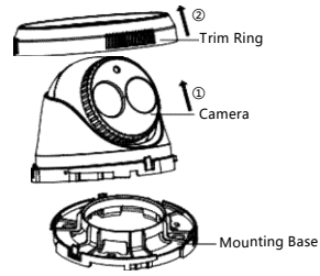
Figure 2-9 Disassemble the Camera
