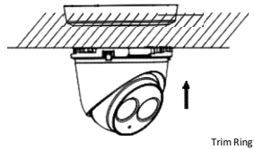
Figure 2-22 Install the Trim Ring
