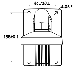
Figure 2-36 Dimension of Demonstrated Wall Mounting Bracket
