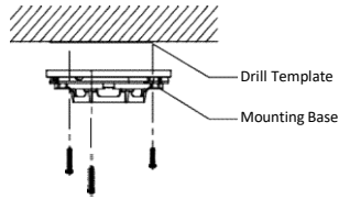
Figure 2-26 Fix Mounting Base
