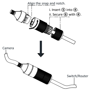
Figure 2-44 Waterproof Accessory Installation
