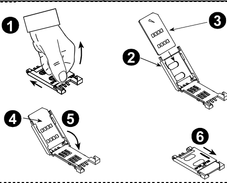
Figure 4 SIM card insertion
