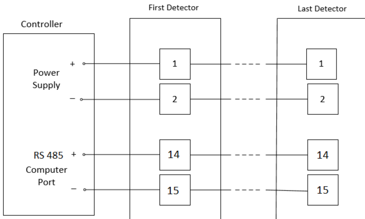
Figure 8: RS-485 Networking
