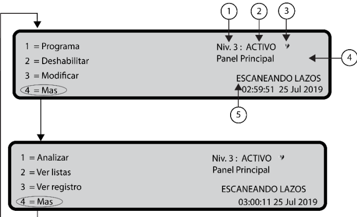
Figura 19: Pantalla PRINCIPAL
