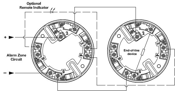
Fig. 1: 2-wire base wiring connections
