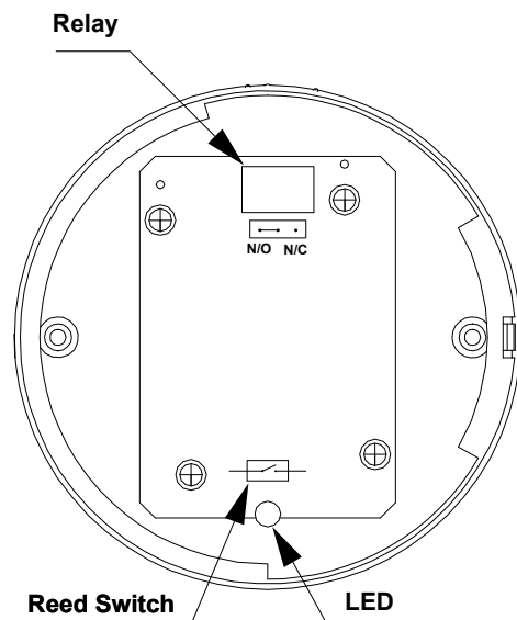
Fig. 3: Adjusting the output relay
