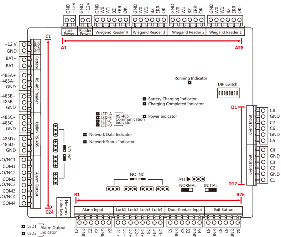
Figure 4-3 Four-Door Access Controller Main Board
