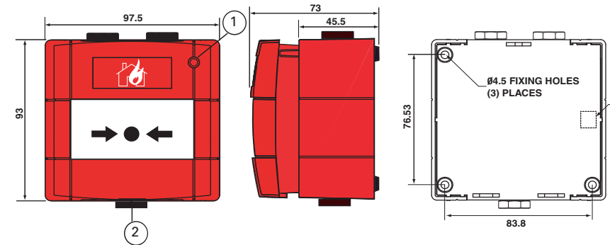
Fig. 1: FC421CP-I Outdoor Weatherproof Resettable Callpoint - Overall and Fixing Dimensions 1– Short Circuit Isolator Activation (Yellow) and Alarm Indicator LED (Red) 2– Test/Release Key Access 3– Earth Continuity Terminal (Internal)
